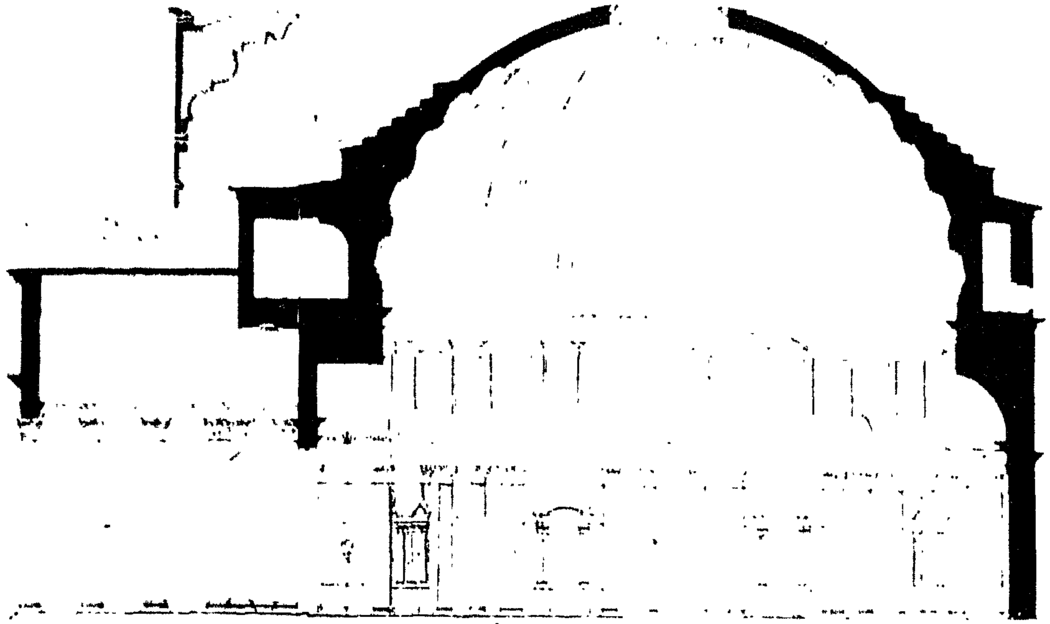
A SECTION THRO' PORTICO AND ROTUNDA
